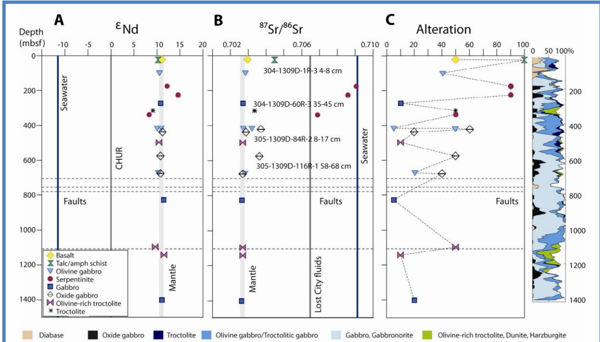
Figure 5.3 Comparison of \epsilon\text{Nd} values, ^{87}\text{Sr}/^{86}\text{Sr} ratios, and alteration with depth and lithostratigraphy at IODP Hole U1309D at the central dome of the Atlantis Massif (from Delacour et al. , 2008a). Depths of fault gouges identified by the IODP Shipboard Scientific Party are shown as horizontal dashed lines (695, 756, 785 and 1107 mbsf; Expedition Scientific Party, 2005a; 2005b; Blackman et al. , 2006). Sr isotope composition of the Lost City end-member fluid (from Ludwig et al. , 2006).
