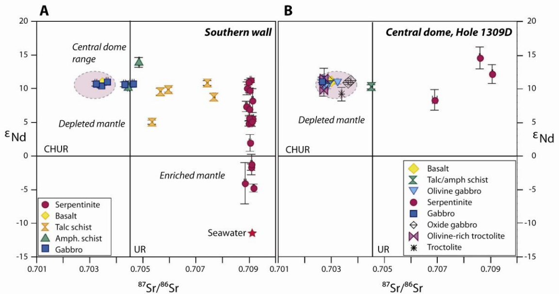
Figure 5.4 Variation in \epsilon\text{Nd} versus ^{87}\text{Sr}/^{86}\text{Sr} for samples [A] from the southern wall of the Atlantis Massif and [B] drilled at IODP Hole U1309D of the central dome. The internal error-bars (2s), the \epsilon\text{Nd} composition of the CHUR (Chondritic Uniform Reservoir of 0.512638), and the Sr isotope composition of the UR (Uniform Reservoir of 0.7045) are shown for reference (from Delacour et al. , 2008a).
